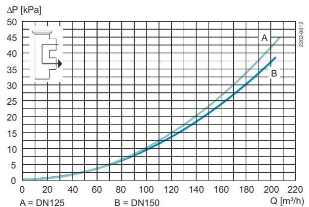
Figure 6. Change-over valve
