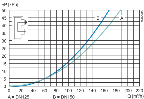
Figure 7. Change-over valve
