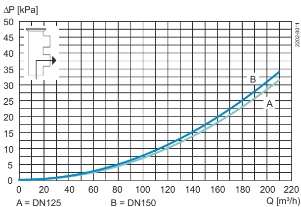
Figure 5. Change-over valve
