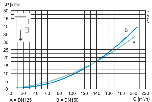
Figure 8. Change-over valve
