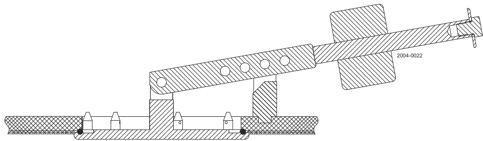
Figure 1. Integrated Valve
