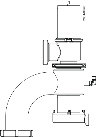
Figure 1. Anti Vacuum House with CO2 House
