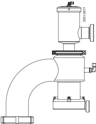
Figure 2. Anti Vacuum House with Pressure Exhaust
