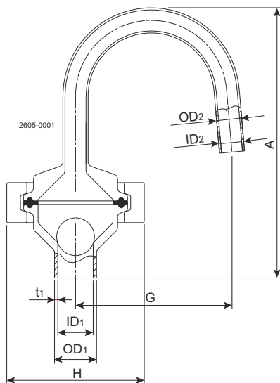
Figure 1. Dimensions
