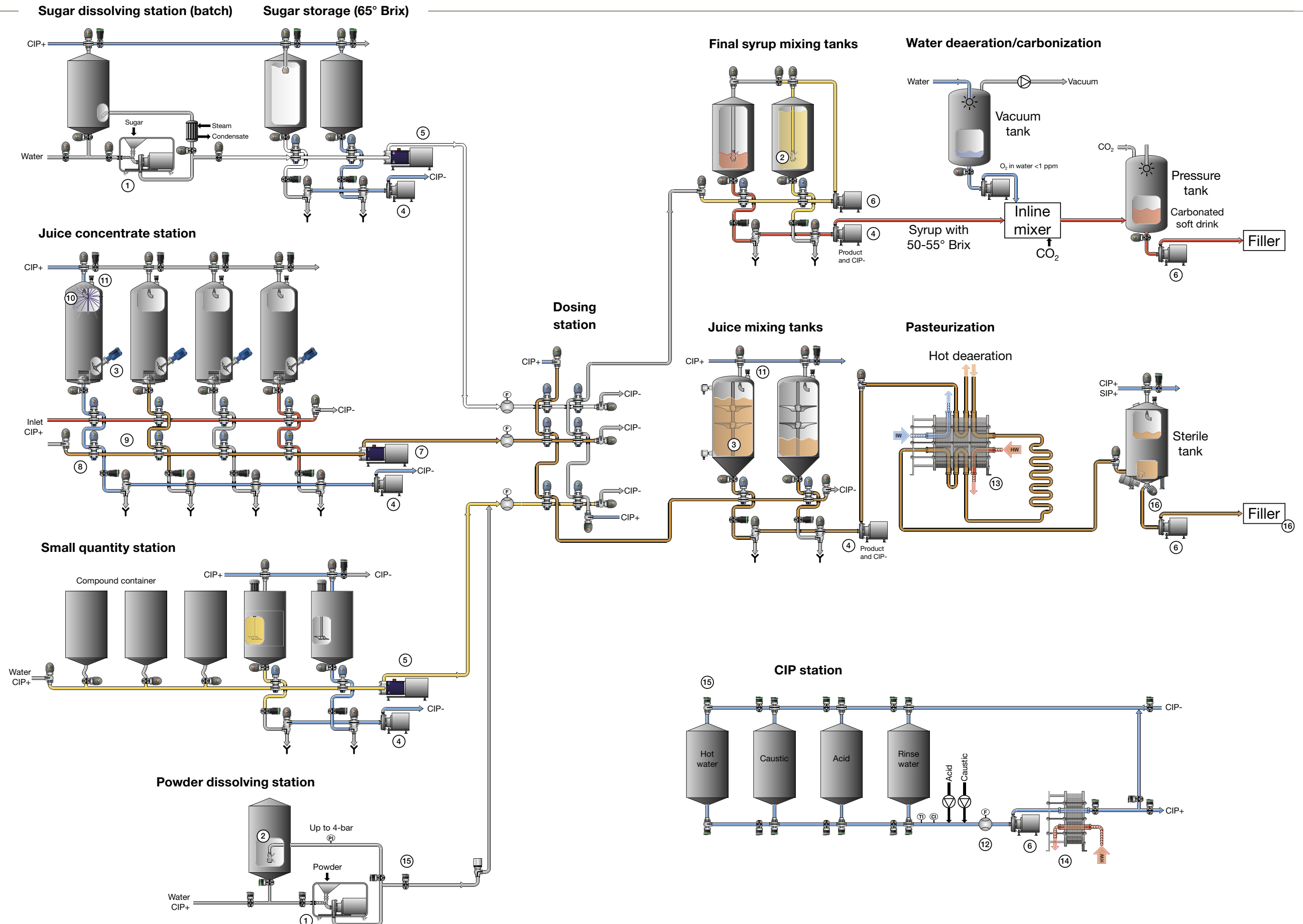
Schematic process chart
